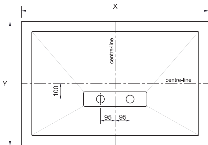
Position of waste holes relative to the centre of each tray.
